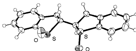
Figure 1. ORTEP diagram of bis(sulfoxide) 6
