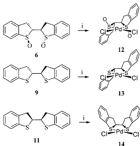
Scheme 5. Preparation of complexes 12–14 ; reagents and conditions: (i) \text{PdCl}_2 , \text{CH}_2\text{Cl}_2 , room temp. (quant.)
