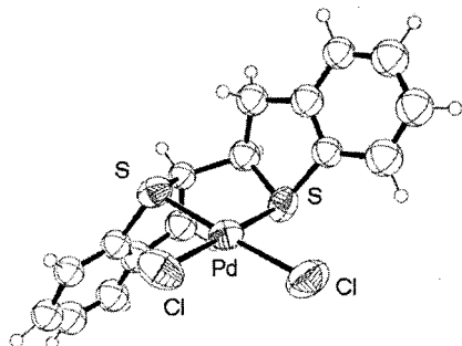
Figure 2. ORTEP diagram of complex 13
