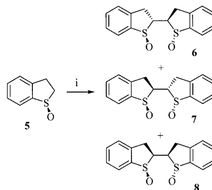
Scheme 3. Synthesis of bis(sulfoxide)s 6–8 ; reagents and conditions: (i) a: LDA, THF, −78 °C. b: CuCl 2 , −78 °C → room temp. c: O 2 , 76%, 1:1:1 diastereomeric ratio
