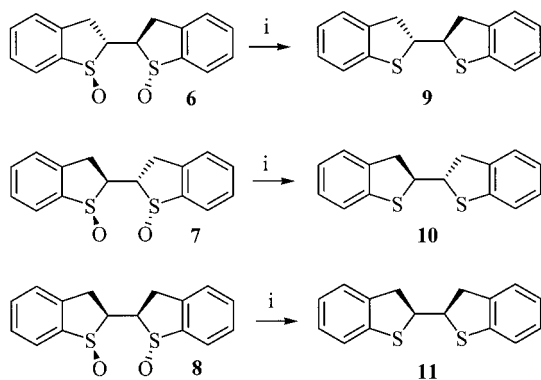
Scheme 4. Synthesis of bis(thioether)s 9–11 ; reagents and conditions: (i) \text{BH}_3 \cdot \text{THF} , THF, 0^\circ\text{C} \rightarrow \text{room temp.} (quant.)
