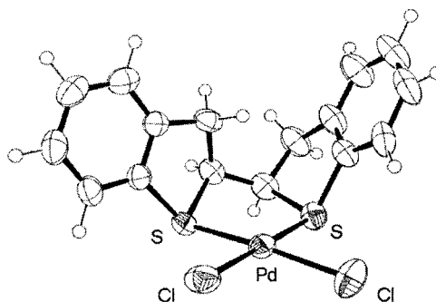
Figure 3. ORTEP diagram of complex 14
