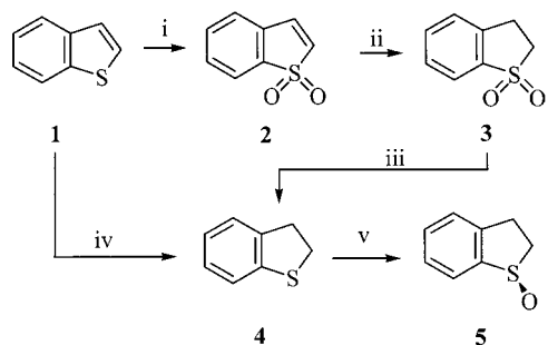
Scheme 2. Preparation of ( R )-2,3-dihydrobenzo[ b ]thiophene 1-oxide ( 5 ); reagents and conditions: (i) m -CPBA, CHCl 3 , room temp., 19 h (90%); (ii) H 2 , 1 atm, 10% Pd/C (quant.); (iii) LiAlH 4 , Et 2 O, reflux, 4 h (77%); (iv) H 2 , 30 atm, [Ru II (triphos)(MeCN) 3 (OTf) 2 ], THF, 100 °C (96%); (v) CPO, H 2 O 2 , pH 5 buffer, room temp., 22 h (90%, 98% ee )
