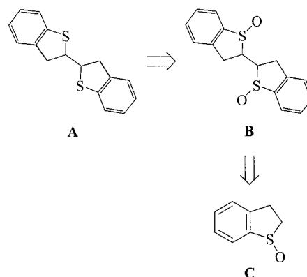
Scheme 1. New approach for the preparation of SCCS-type ligands
